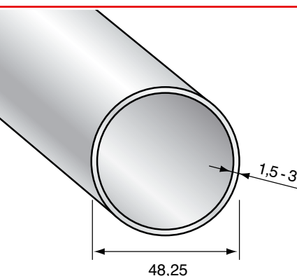
Art. P 0479G grezzo € 10,50/mt. Art. P 0479A argento € 13,65/mt. Tubo in alluminio, Ø 48,25mm, spess. 1,5 mm. Barre da 3-6 mt.
