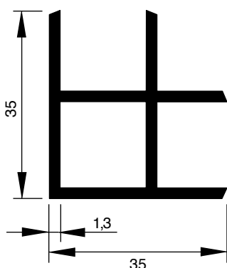
Art. P7302A-M6 argento € 9,50/mt.
